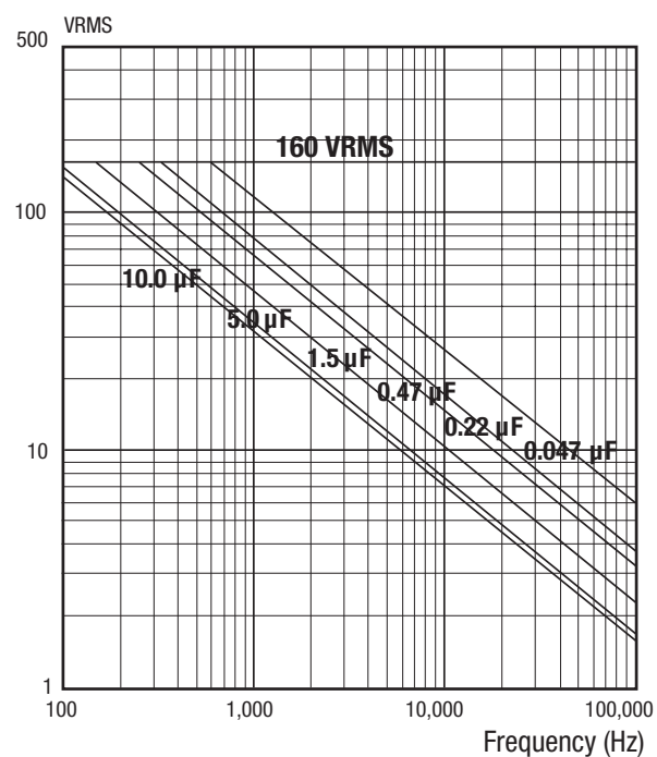
VOLTAGE VS. FREQUENCY TYPE 442P 250 VDC / 160 VAC
