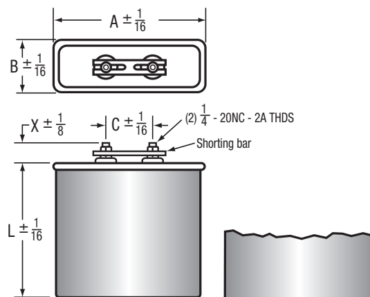
FIGURE 1 DRAWN CASE
