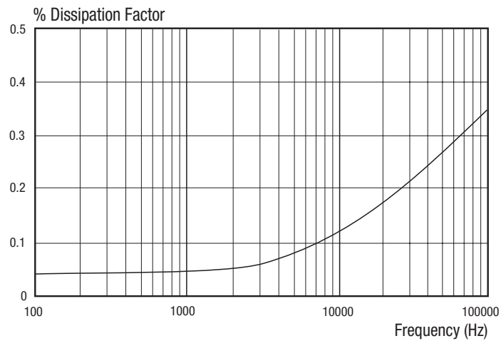
DISSIPATION FACTOR VS. FREQUENCY - METALIZED POLYPROPYLENE
