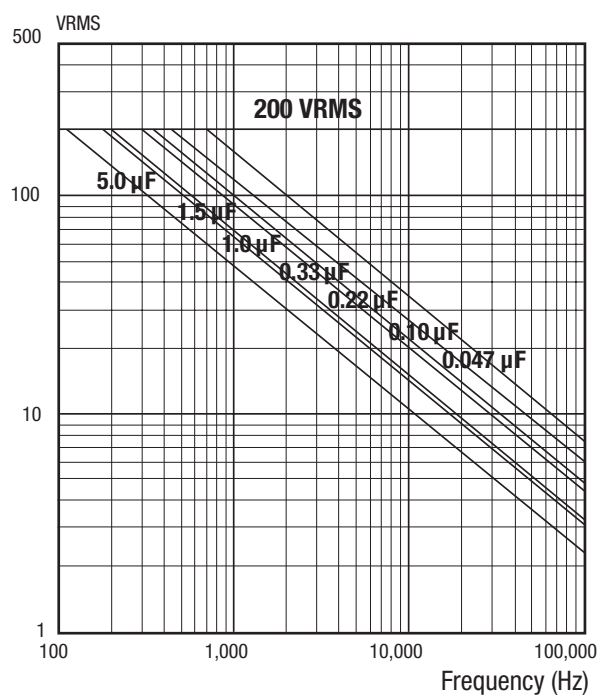
VOLTAGE VS. FREQUENCY TYPE 442P 400 VDC / 200 VAC
